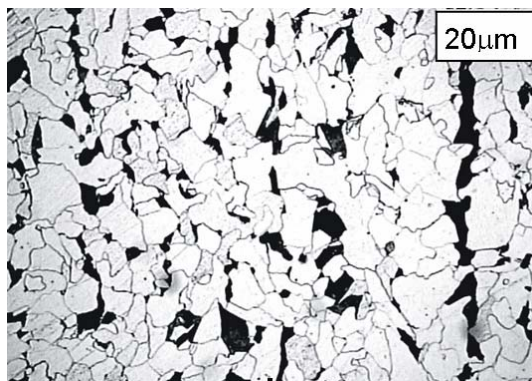
Fig.2 Optical metallograph of steel microalloyed with V
